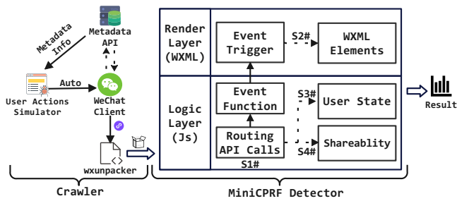
Figure 5: The Workflow of MINICAT.
